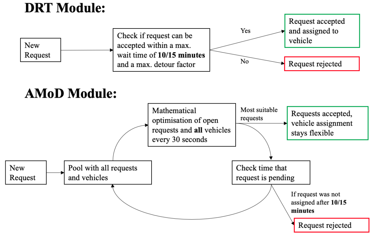
Figure 2: Booking Process in the DRT and the AMoD module
